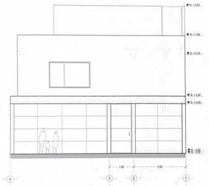
ALZADO PRINCIPAL
